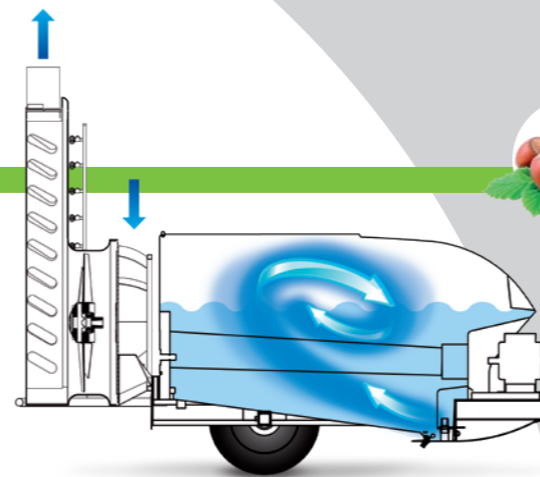
Serbatoio con pendenza anteriore (mod.1500) Tank with the front slope. (mod.1500) Nach vorne geneigter Tank. (mod.1500)
